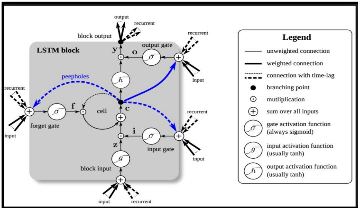
Figure 6: LSTM model's memory cell architecture
