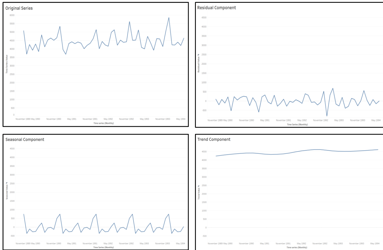
Figure 5. Splitting the time series into seasonal, trend and noise components
